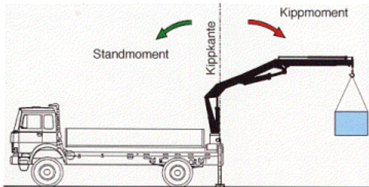
Abb. 21: Standmoment, Kippmoment
